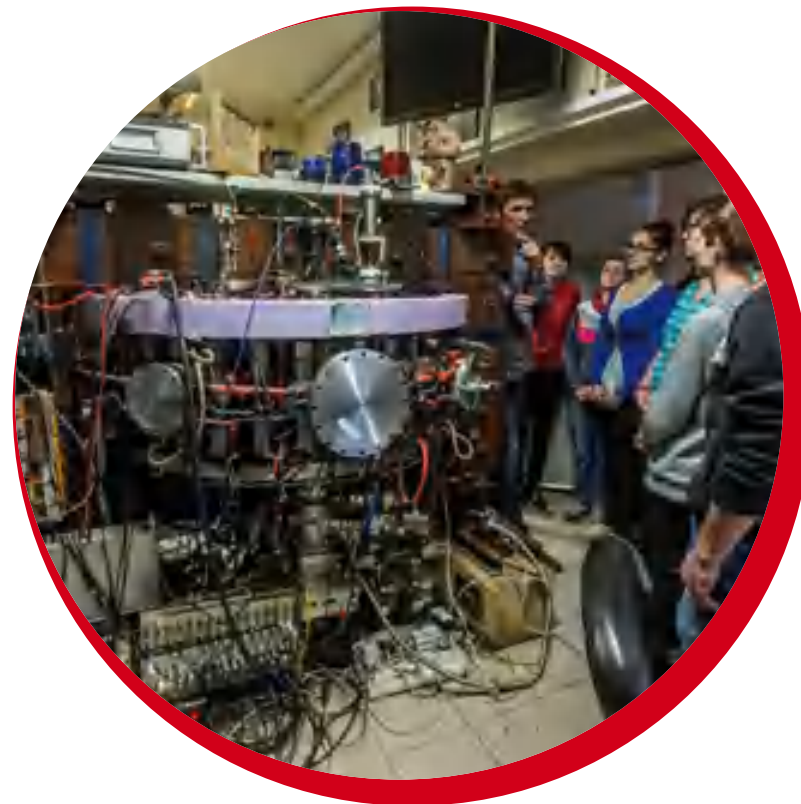
GOLEM tokamak - Czech Technical University in Prague
